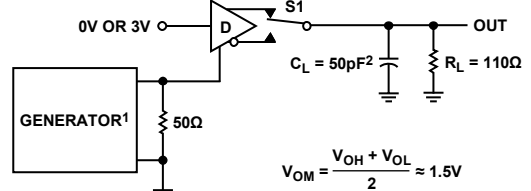
Figure 13. Driver Enable and Disable Times ( t_{PZH} , t_{PSH} , t_{PHZ} )
